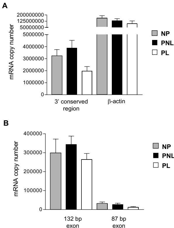
Figure 2 Maxi-K \alpha subunit mRNA expression analysed by quantitative real-time PCR. Results shown represent mean ( \pm standard error of the mean, SEM) copy number values for (A) total Maxi-K \alpha subunit (represented by the 3' conserved region), and \beta -actin, and (B) the 132 bp and 87 bp alternatively spliced exons of the Maxi-K \alpha subunit. Copy number values were obtained based on product-specific serially-diluted cDNA standards, generated individually for each amplicon of interest. Tissue sets are indicated by striped columns (non-pregnant, NP), black columns (pregnant not-in-labour, PNL) and open columns (pregnant in-labour, PL).
